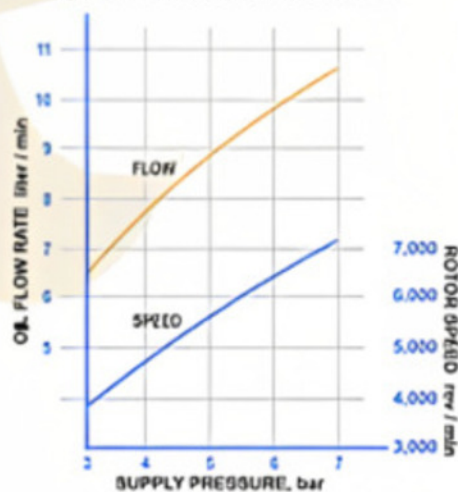
PERFORMANCE CURVES Typical rotor performance for 9AFC 30 OIL @ 15°C
