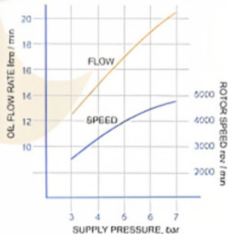
PERFORMANCE CURVES Typical rotor performance for SAE 30 OE @ 75°C
